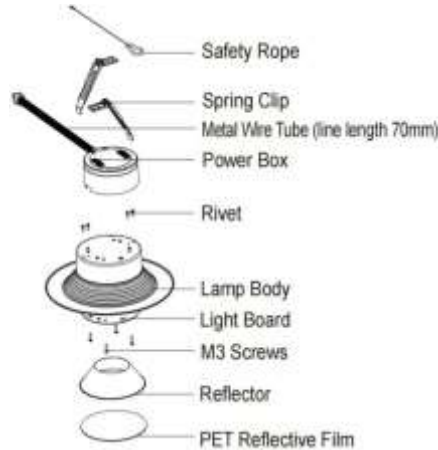
Exploded Drawing
