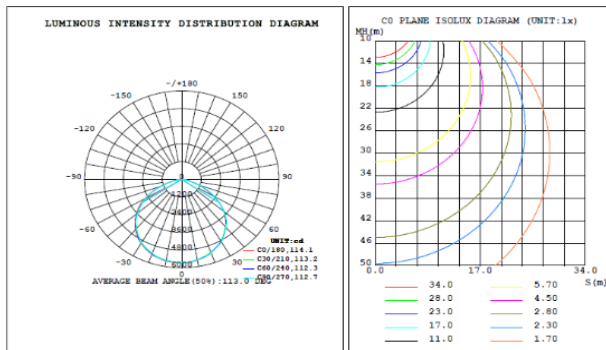
Ø 10.24*6.26 inch 100W
