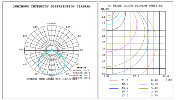
Ø 10.24*6.85 inch 150W
