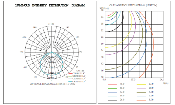
Ø 12.60*6.73 inch 240W
